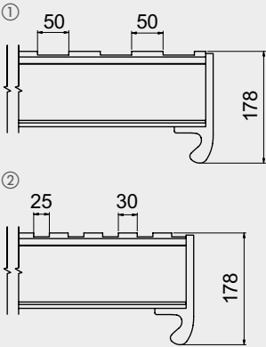
1 STEP 50/50 (STANDARD) 2 SPECIAL STEP 25/30 (ON REQUEST)
