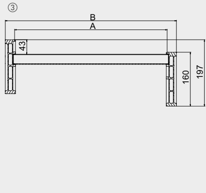
③ WITH ONLY ONE RAISED EDGE
