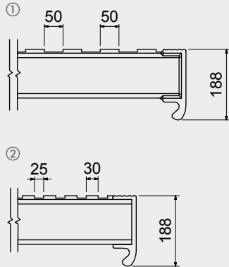
1 STEP 50/50 (STANDARD) 2 SPECIAL STEP 25/30 (ON REQUEST)
